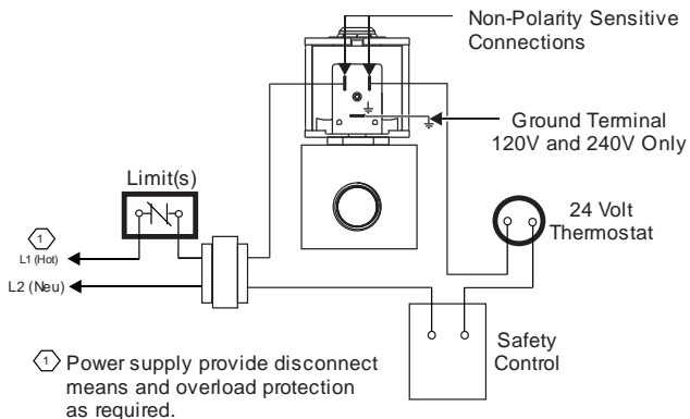
Figure 5: Electrical Connections
