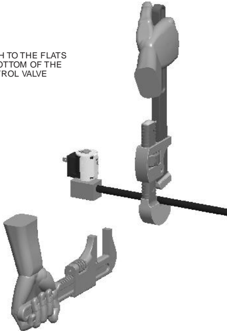
Figure 3: Proper Use of Wrench on Gas Control
