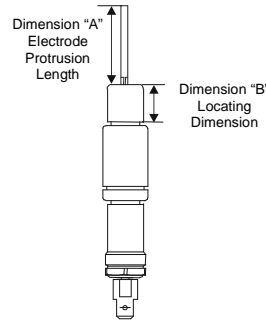
Figure 1: Y75 Sensing Probe
