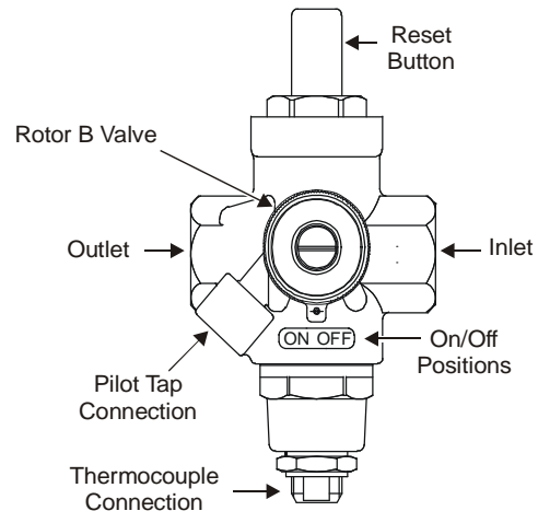
Figure 4: Typical H19 Valve with Rotor Valve
