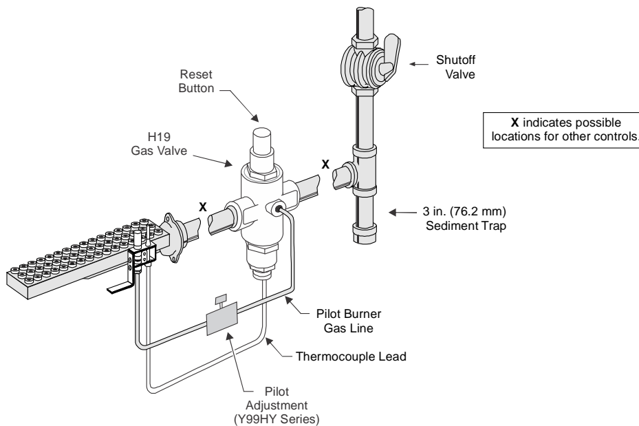
Figure 3: Typical Installation
