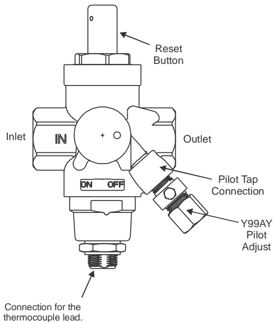
Figure 3: Typical H19 Valve with Manual Pilot Adjust
