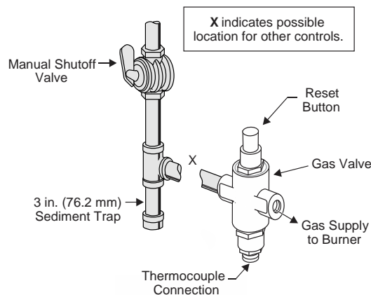
Figure 2: Typical H19ME/H19PE Installation
