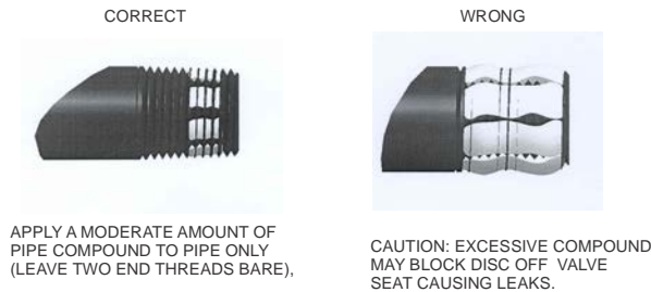
Figure 1: Use a Moderate Amount of Pipe Compound
