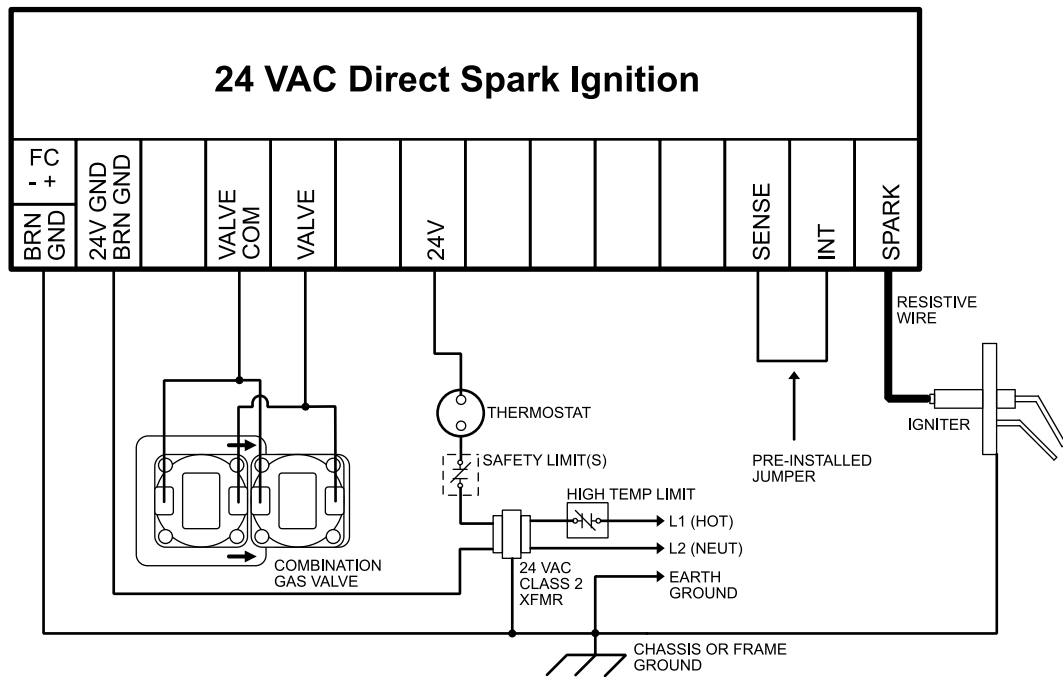
Figure 1: Wiring for 1 Rod Flame Sense used for Local (Internal) Sense
