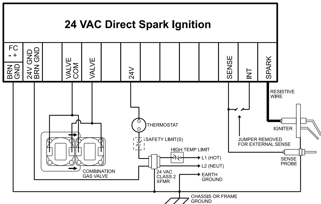
Figure 2: Wiring for 2 Rod Flame Sense used for Remote (External) Sense
