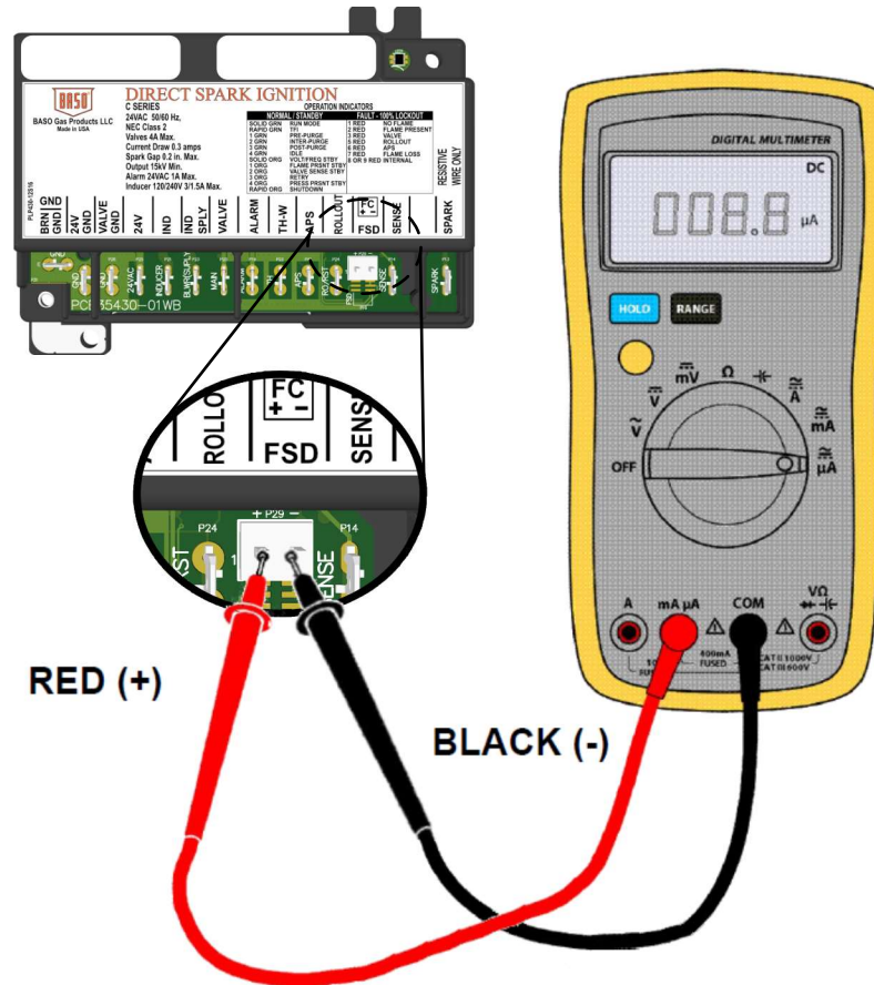
Figure 4: Microammeter Connection
