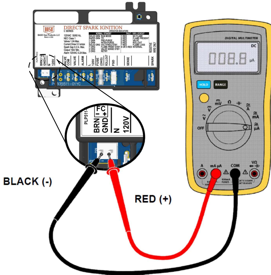
Figure 4: Microammeter Connection
